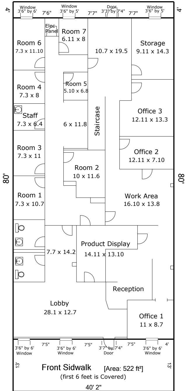
First Floor [Area: 3213 ft 2 ]
