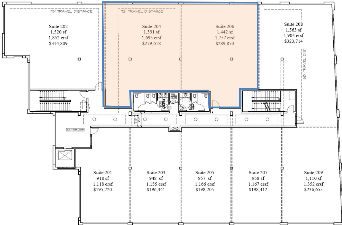
2 A.1 SECOND FLOOR PLAN SCALE: 3/32" = 1'-0"
